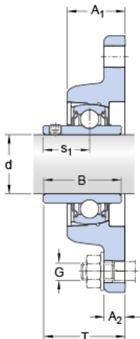
FYT 40 TF/VA228 Bearing 2D drawings and 3D CAD models
